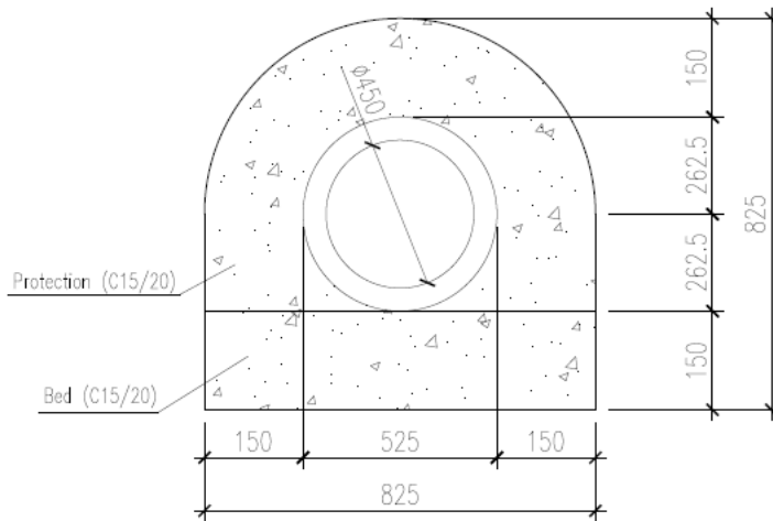
0.450m Dia. Storm Pipe Detail
